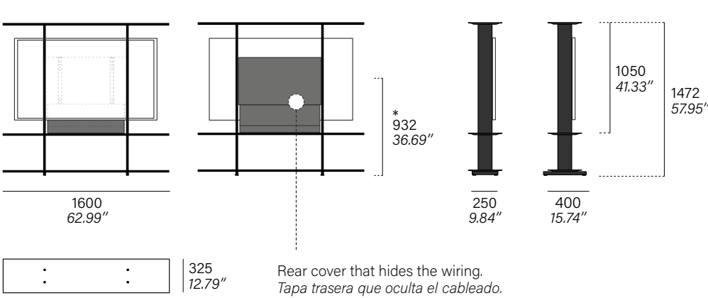
1600 Home Basic TV stand
