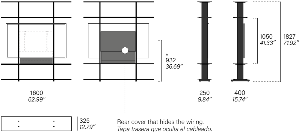
1600 Home TV stand
